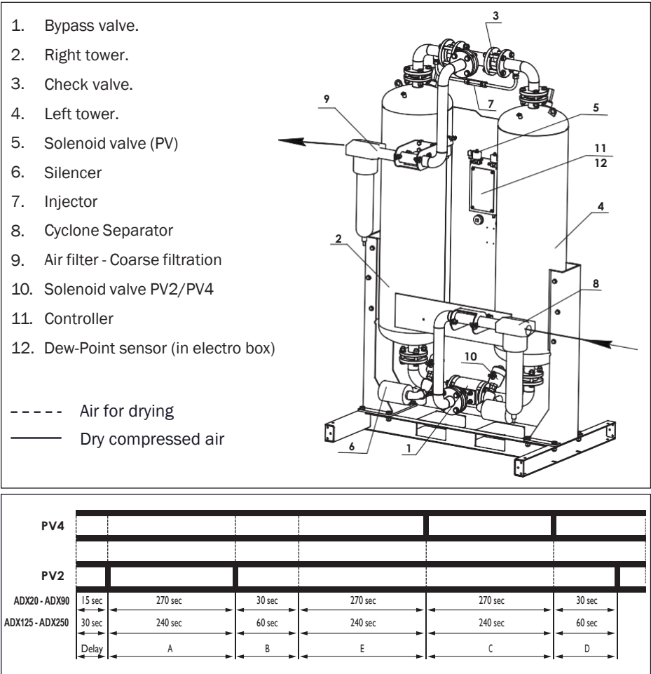
Fig. 2.3 Flow chart of air dryer
